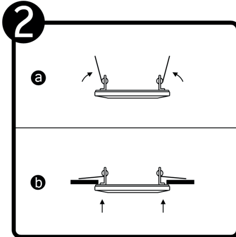
Option 1 Ø 129mm MINIMUM
